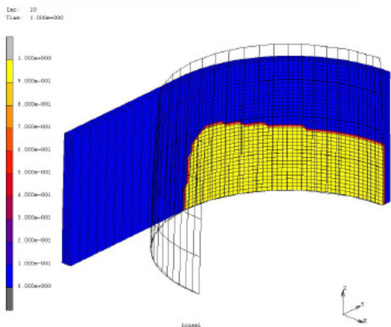
Contact area with pulley diameter 34 mm Crowning radius 250
