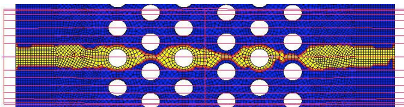
Contact surface area of PES-belt with e-modulus 1613 N/mm 2
