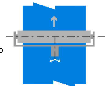
Tensioning-/ tail roll and tracking idler
