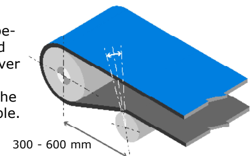
Tensioning-/ tail roll and tracking idler
